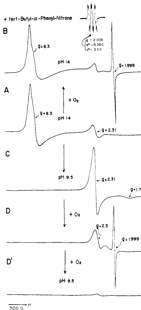
Figure 2. (A) Iron oxymesoporphyrin ( 6b ; \sim 1 mM) in 60% aqueous pyridine solution containing 0.4 N NaOH; (B) air was bubbled through A and spin trapped with tert-butyl- \alpha -phenylnitron ; (C) pH of A was adjusted to 9.5 anaerobically by adding barbituric acid; (D) trace of air was introduced to C; (D') air was bubbled through D for another 1 min. ESR spectra were recorded with a JES-FE-3X spectrometer operating with 100-kHz magnetic field modulation.
